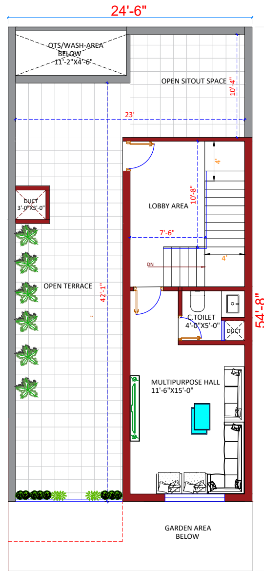
MAIN ROAD SECOND FLOOR PLAN
